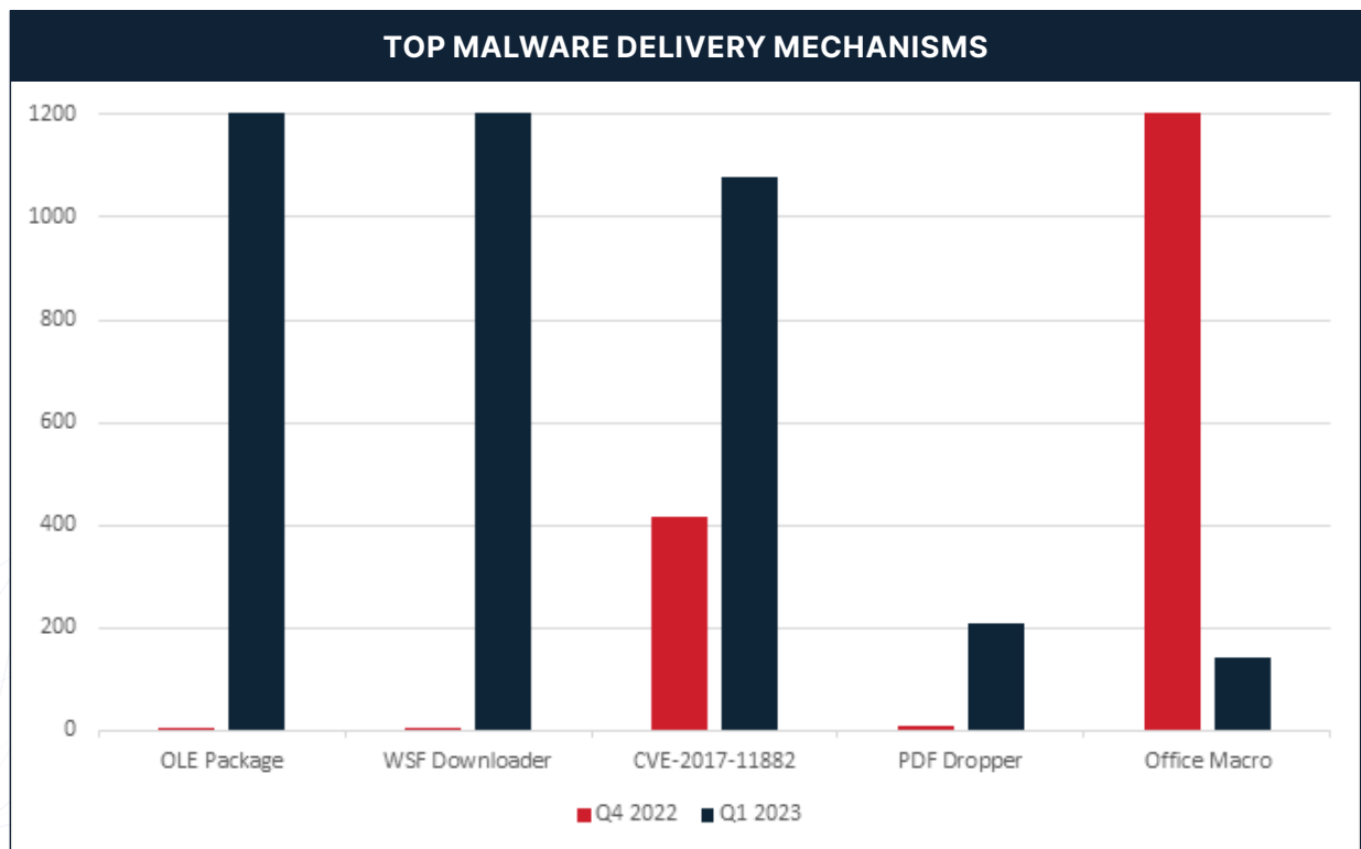
Figure 5: Top Malware Delivery Mechanisms by Email Volume in Q4 2022 and Q1 2023. The maximum values for the chart are capped, and do not show the full volume of mechanisms associated with Emotet.
