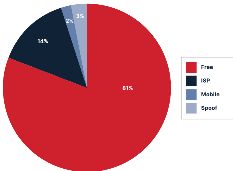
FIGURE 7: BEC DOMAINS
